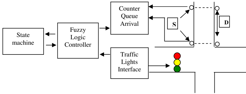
Figure 2 General structure of a fuzzy input/output traffic lights Control System
